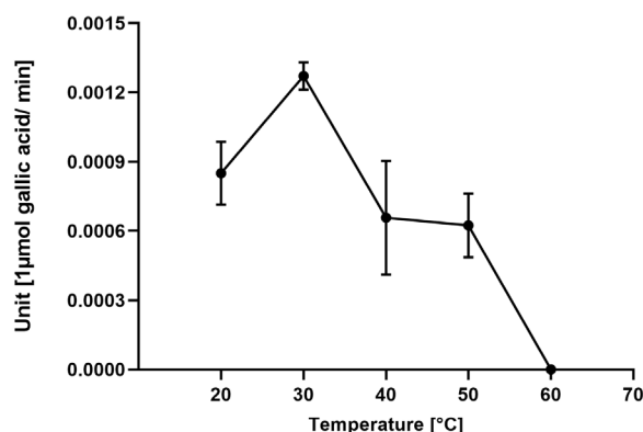
Figure 6. Effect of temperature on the activity of the tannase purified from M. corticolus SZMC 12031. Error bars represent the standard deviation.
