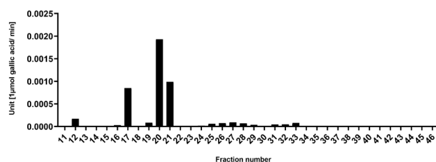
Figure 5. Tannase activity in fractions collected during M. corticulus SZMC 12031 tannase protein purification by anion exchange chromatography.
