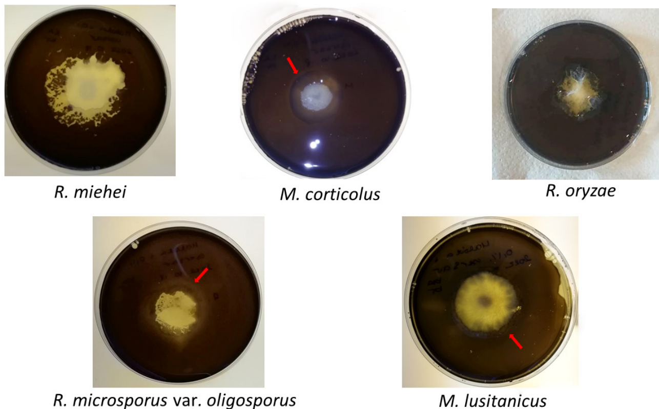
Figure 1. Study of tannase production by Mucoromycota fungi on tannic acid-supplemented medium. Cultivation was performed in malt extract agar medium (yeast extract 0.25 m/v%, malt extract 0.5 v/v% from 20 v/v% stock solution, glucose 1 m/v%, agar 2 m/v%) supplemented with 0.1 m/v% tannic acid. Plates were stained with 0.01 M iron(III) chloride solution.
