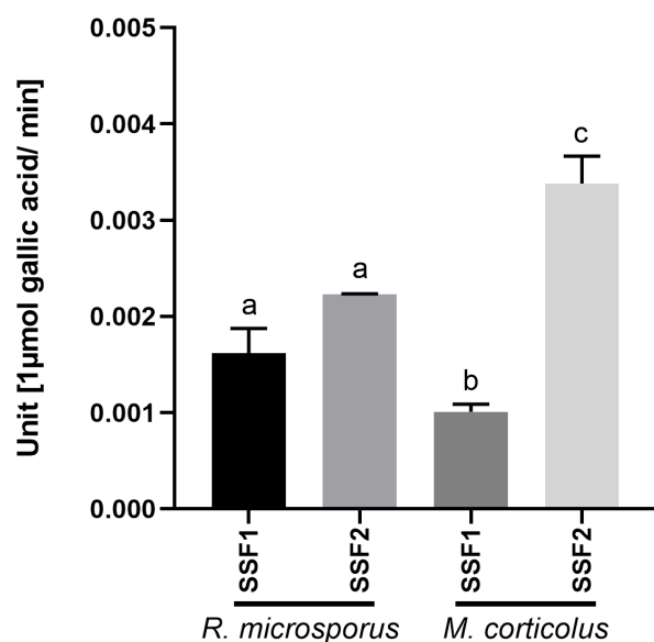
Figure 4. Comparative evaluation of tannase yields of R. microsporus var. oligosporus and M. corticulus achieved in wheat bran-based SSF1 and SSF2 systems. In SSF2 condition, the wheat bran was moisturized with four times the amount of water to that used in SSF1. After 120 h (SSF1) or 72 h (SSF2) incubation, extracts were made using 30 ml (SSF1) or 60 ml (SSF2) sodium acetate buffer. Error bars represent the standard deviation. Different letters above the columns indicate significant differences according to one-way ANOVA ( p < 0.05 ).
