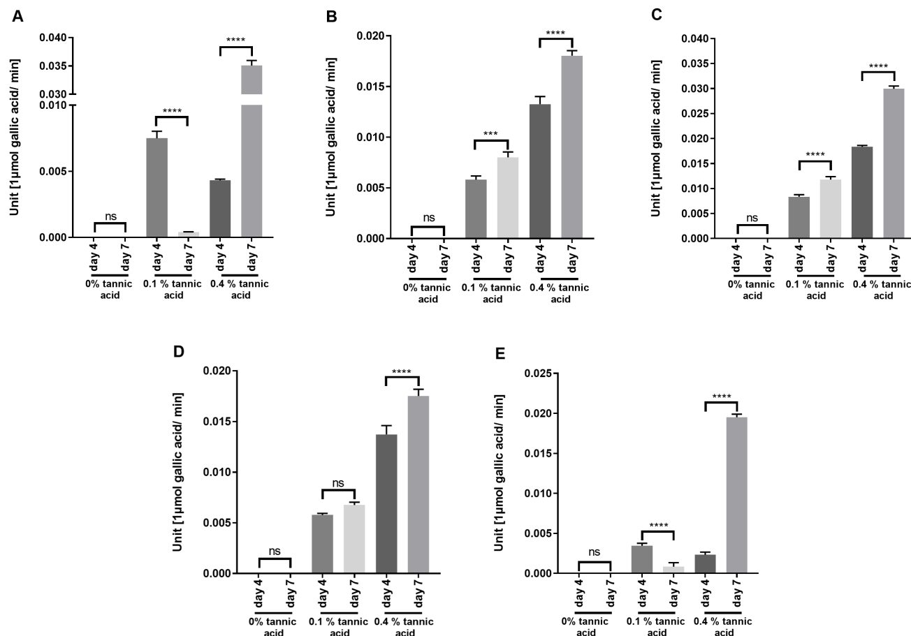
Figure 2. Tannase activity of R. miehei SZMC 11005 (A), M. corticolus SZMC 12031 (B), R. oryzae SZMC 13611 (C), R. microsporus var. oligosporus SZMC 13622 (D) and M. lusitanicus SZMC 12028 (E) strains in submerged fermentations using inducer tannic acid at different concentrations. Error bars represent the standard deviation. Significance was calculated by one-way ANOVA followed by Tukey's multiple comparison test; * p < 0.05 , ** p < 0.01 , *** p < 0.001 , **** p < 0.0001 , ns: non-significant ( p > 0.05 ).
