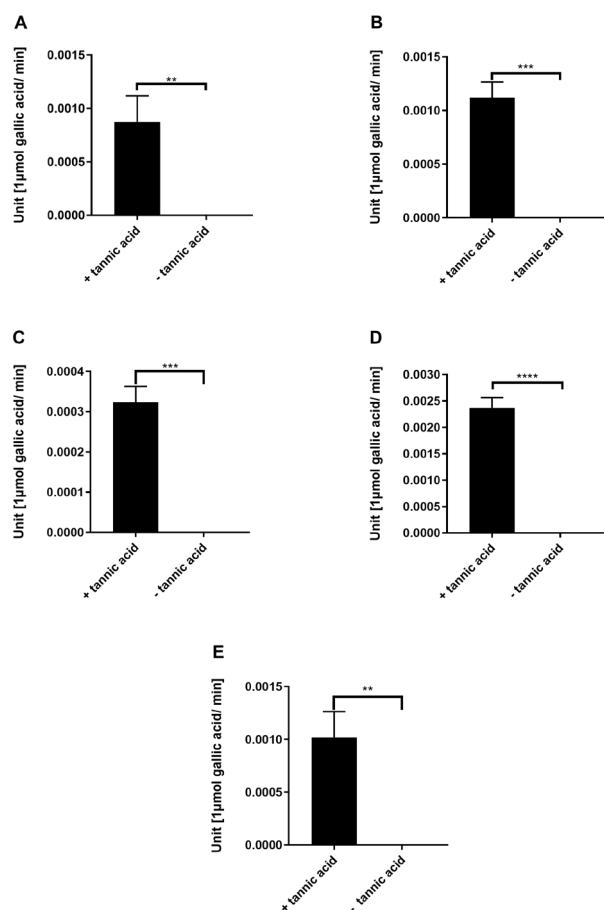
Figure 3. Tannase activity of R. miehei SZMC 11005 (A), M. corticolus SZMC 12031 (B), R. oryzae SZMC 13611 (C), R. microsporus var. oligosporus SZMC 13622 (D) and M. lusitanicus SZMC 12028 (E) strains in wheat bran-based solid-state fermentation. The SSF1 system consisted of 5 g of wheat bran moisturized with Czapek-Dox solution supplemented with tannic acid (+ tannic acid). Tannic acid-free system (- tannic acid) was considered as reference. Error bars represent the standard deviation. Significance was calculated with unpaired t-test; * p < 0.05 , ** p < 0.01 , *** p < 0.001 , **** p < 0.0001 .
